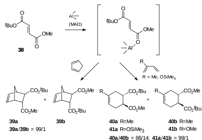
Scheme 10
